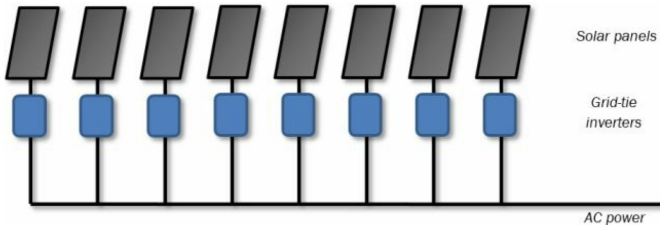
A simplified block diagram showing the basic layout of a micro-inverter system
