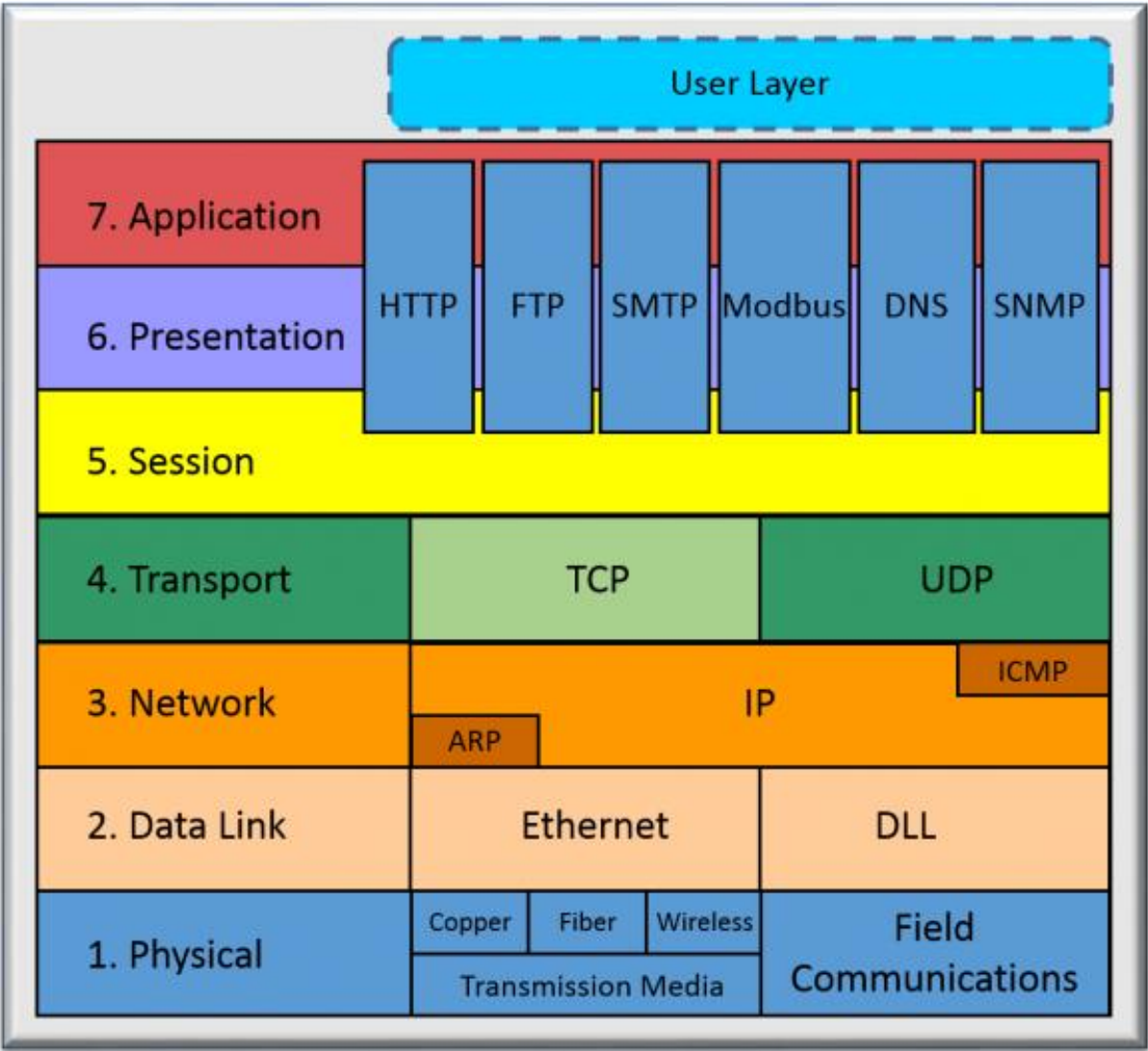
OSI model builds a protocol in layers
